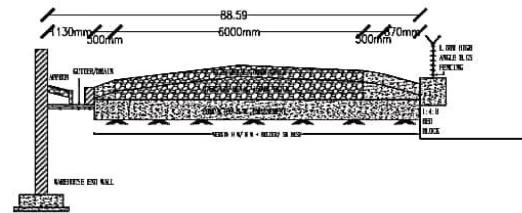
TYPE CROSS SECTION OF ROAD, APPRON, GUTTER/ DRAIN, WIRE FENCING COMPOUND
