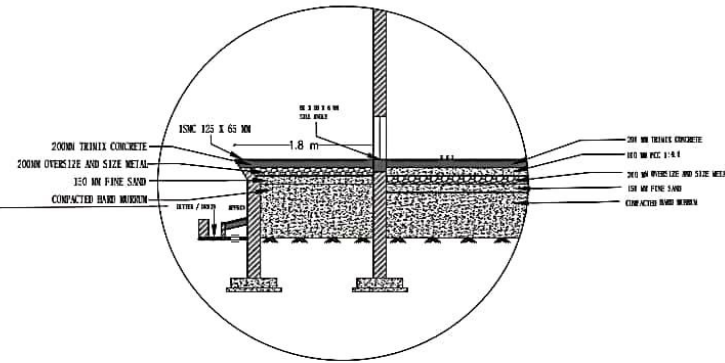
CROSS SECTION PLATFORM
